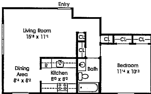
One Bedroom - 550 Sq Ft Garden Level
